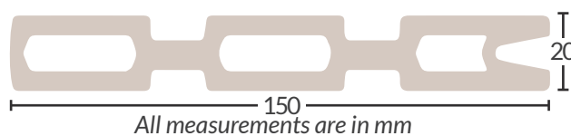
FENCING TOP BOARD
